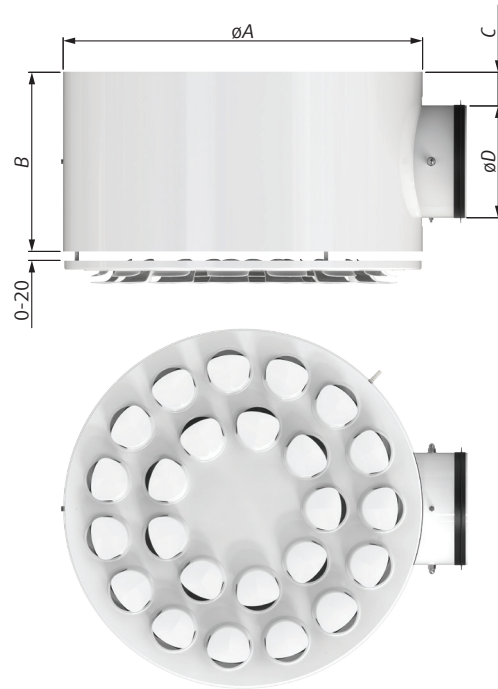
Fig. 1: CAP-C dimensions
